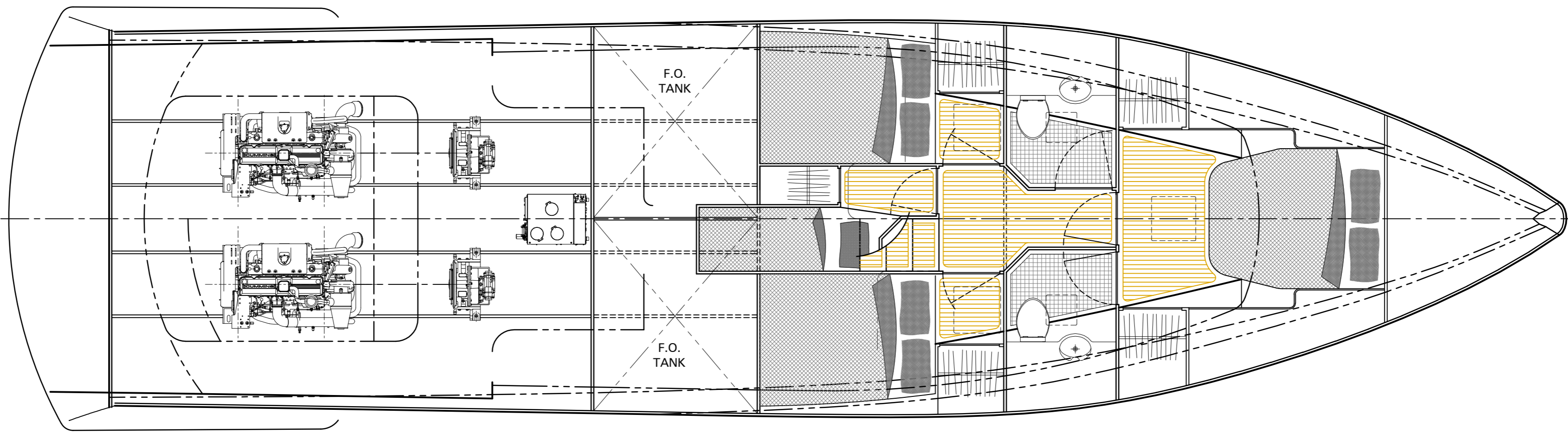
LOWER DECK PLAN
